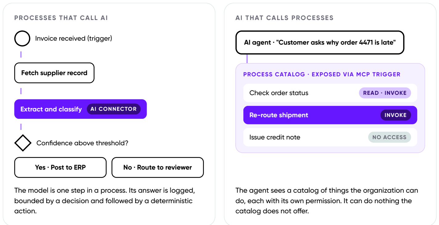
Figure 3. Two directions: AI as a step inside a process, and processes as tools for an AI agent.
