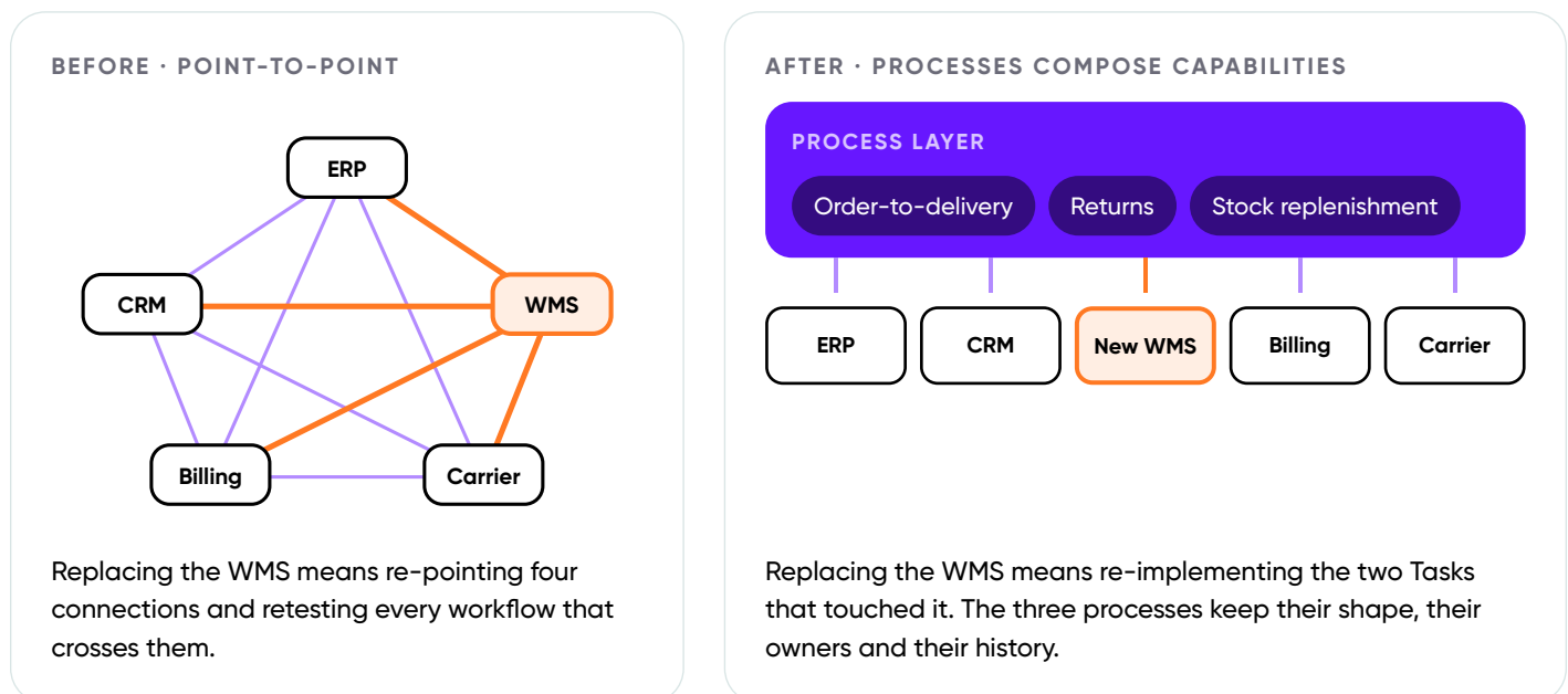
Figure 2. Swap without rebuild: the change is bounded by the steps a system handled, not by everything connected to it.
